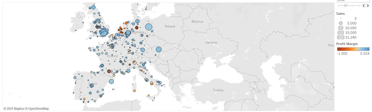
Customer Scatterplot
