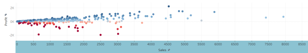
Customer Scatterplot
